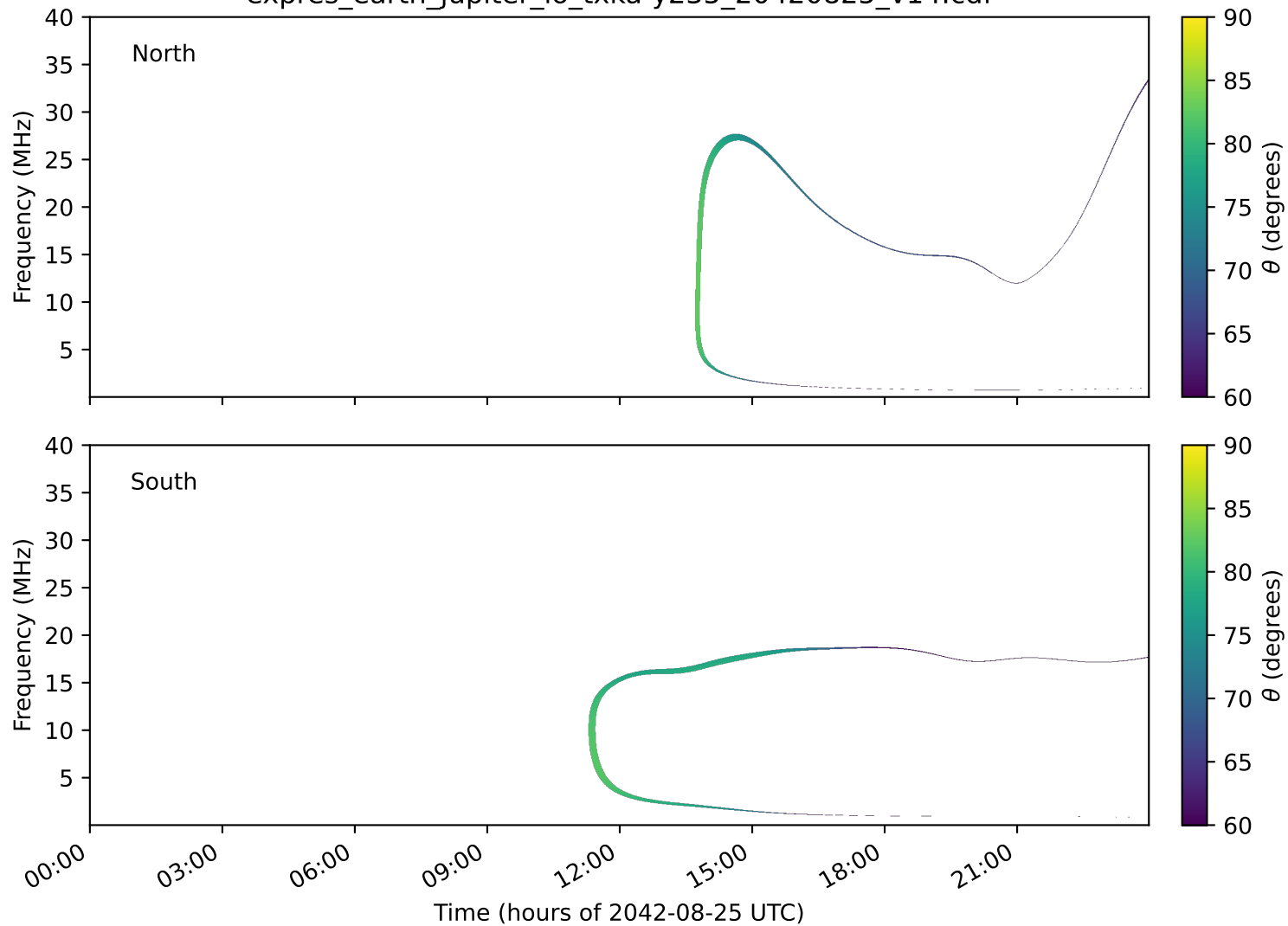
expres_earth_jupiter_io_txka-y235_20420825_v14.cdf
