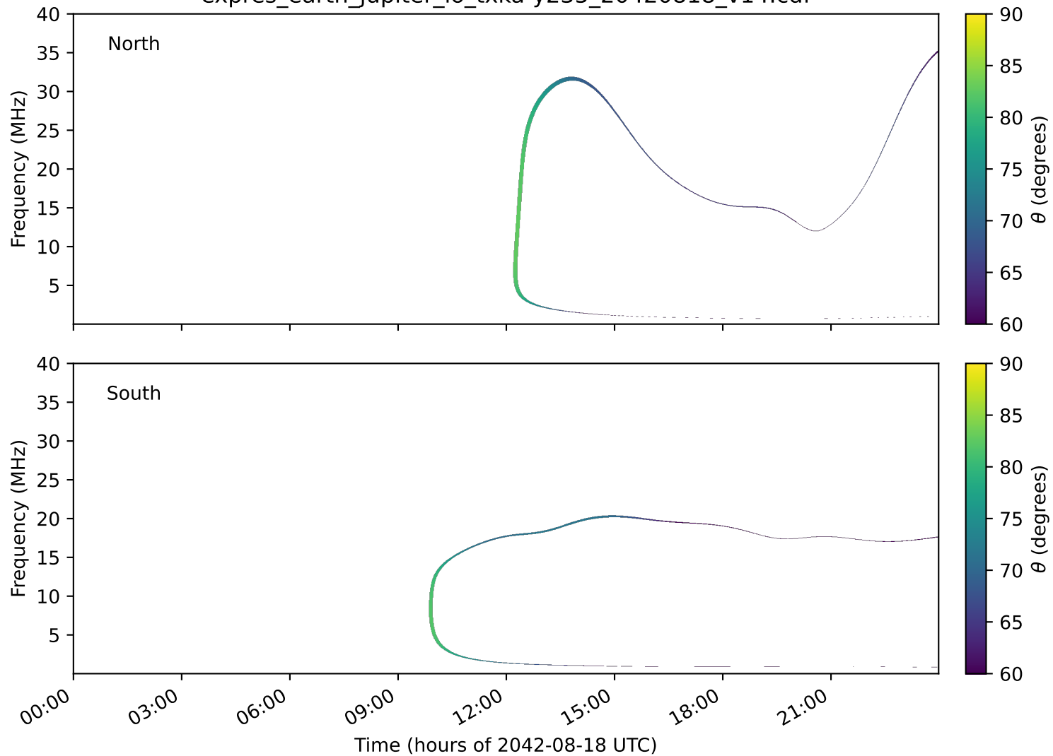
expres_earth_jupiter_io_txka-y235_20420818_v14.cdf
