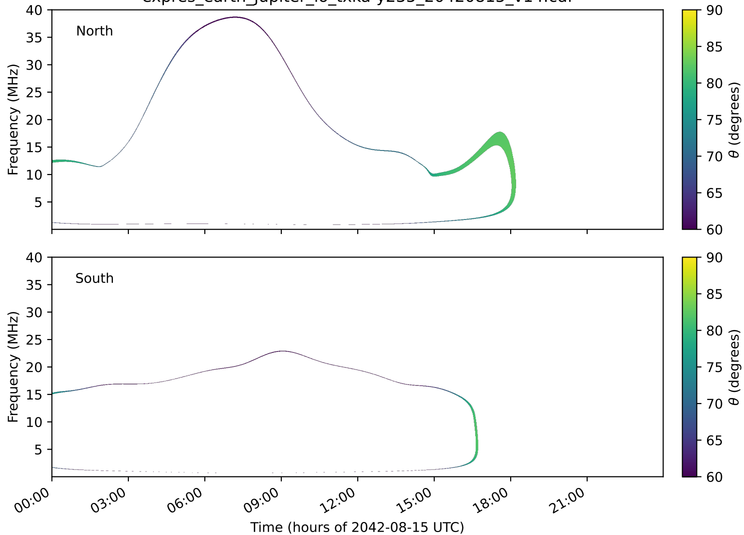
expres_earth_jupiter_io_txka-y235_20420815_v14.cdf
