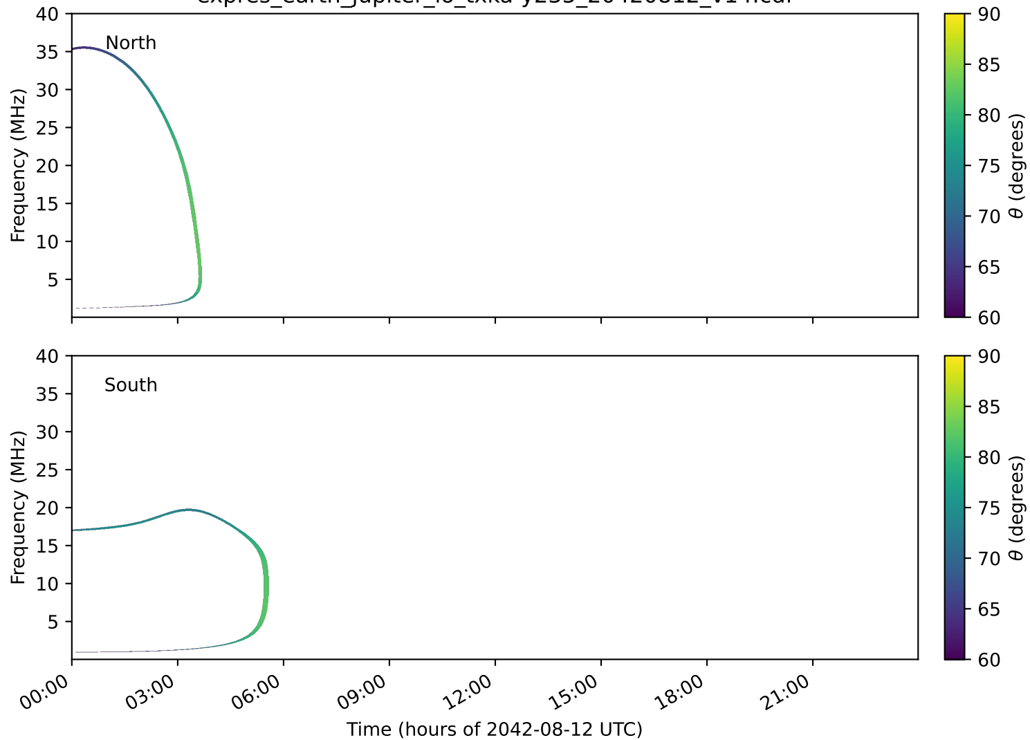
expres_earth_jupiter_io_txka-y235_20420812_v14.cdf
