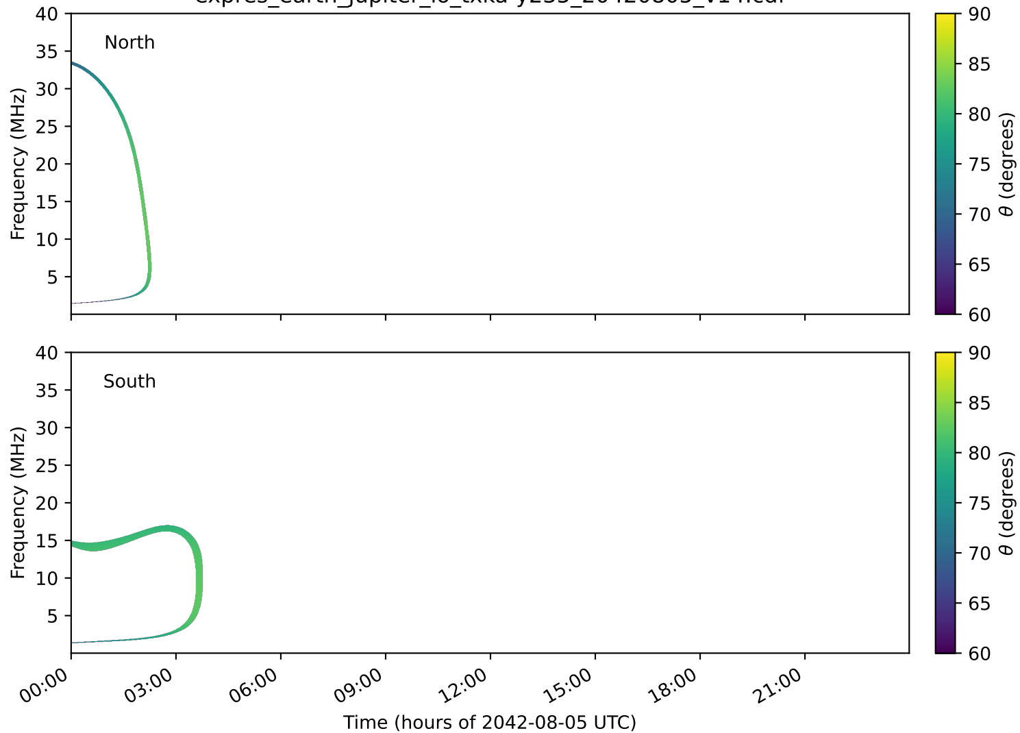
expres_earth_jupiter_io_txka-y235_20420805_v14.cdf
