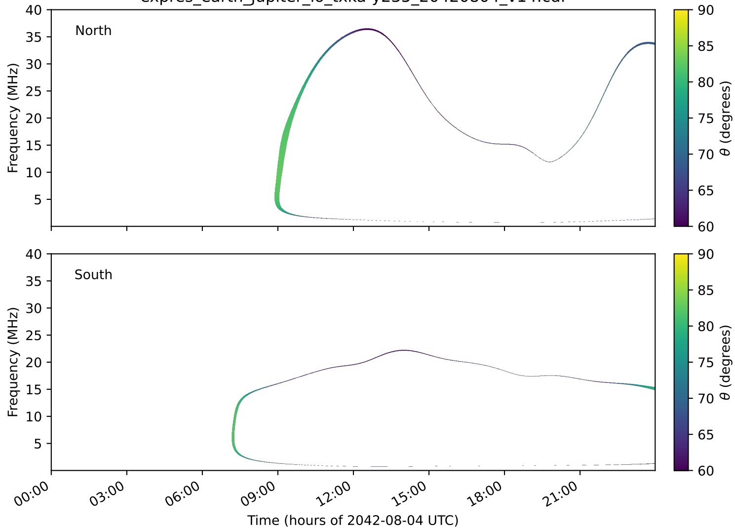
expres_earth_jupiter_io_txka-y235_20420804_v14.cdf
