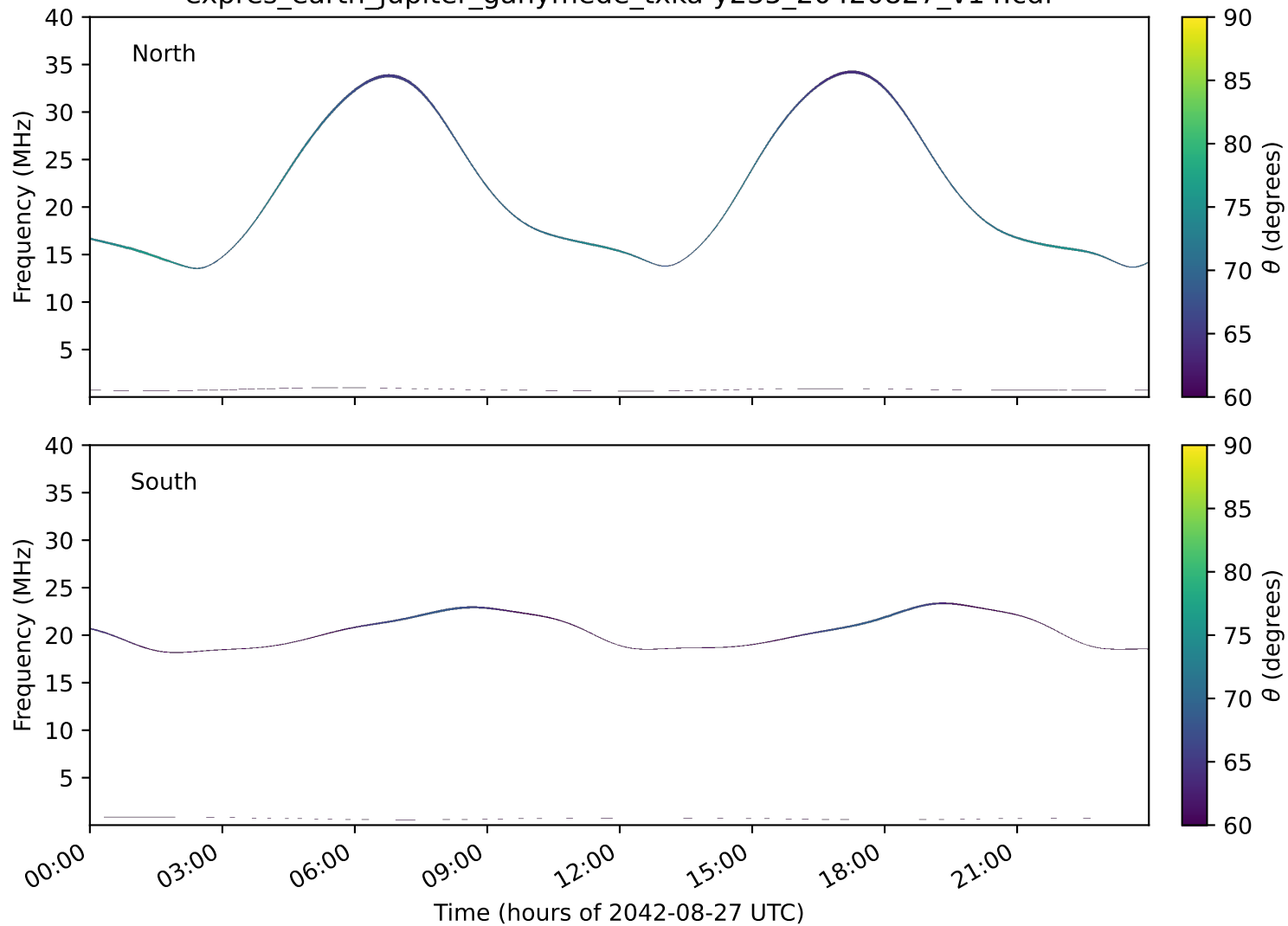
expres_earth_jupiter_ganymede_txka-y235_20420827_v14.cdf
