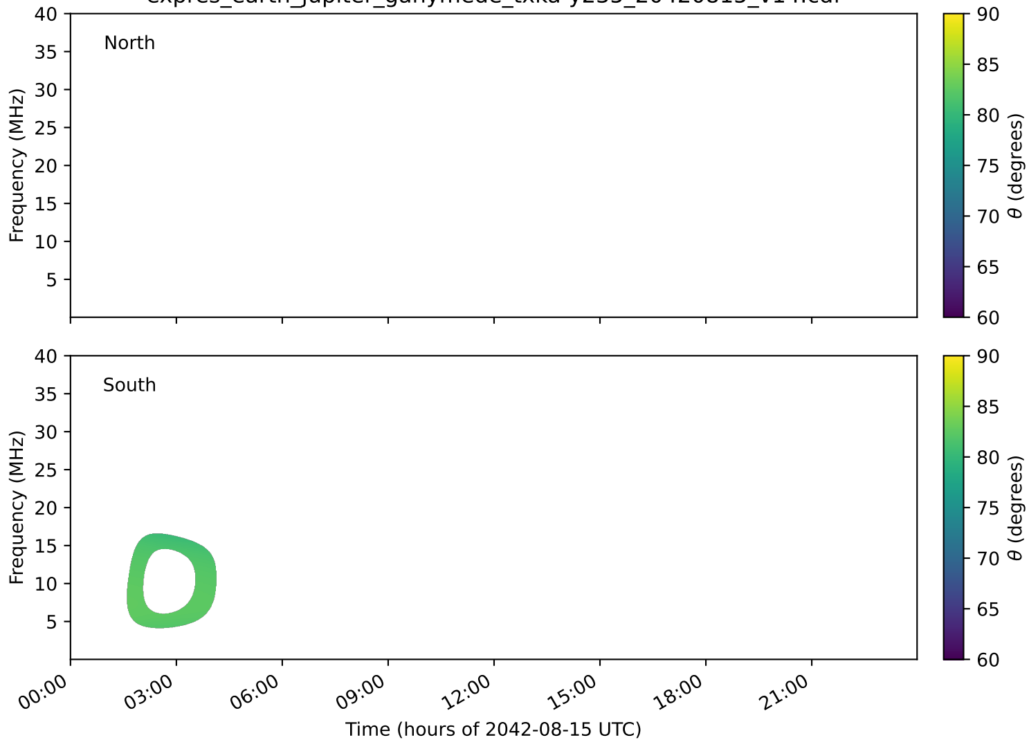
expres_earth_jupiter_ganymede_txka-y235_20420815_v14.cdf
