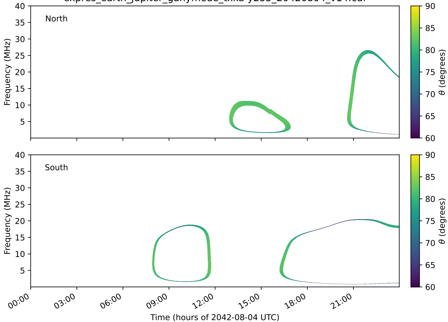
expres_earth_jupiter_ganymede_txka-y235_20420804_v14.cdf
