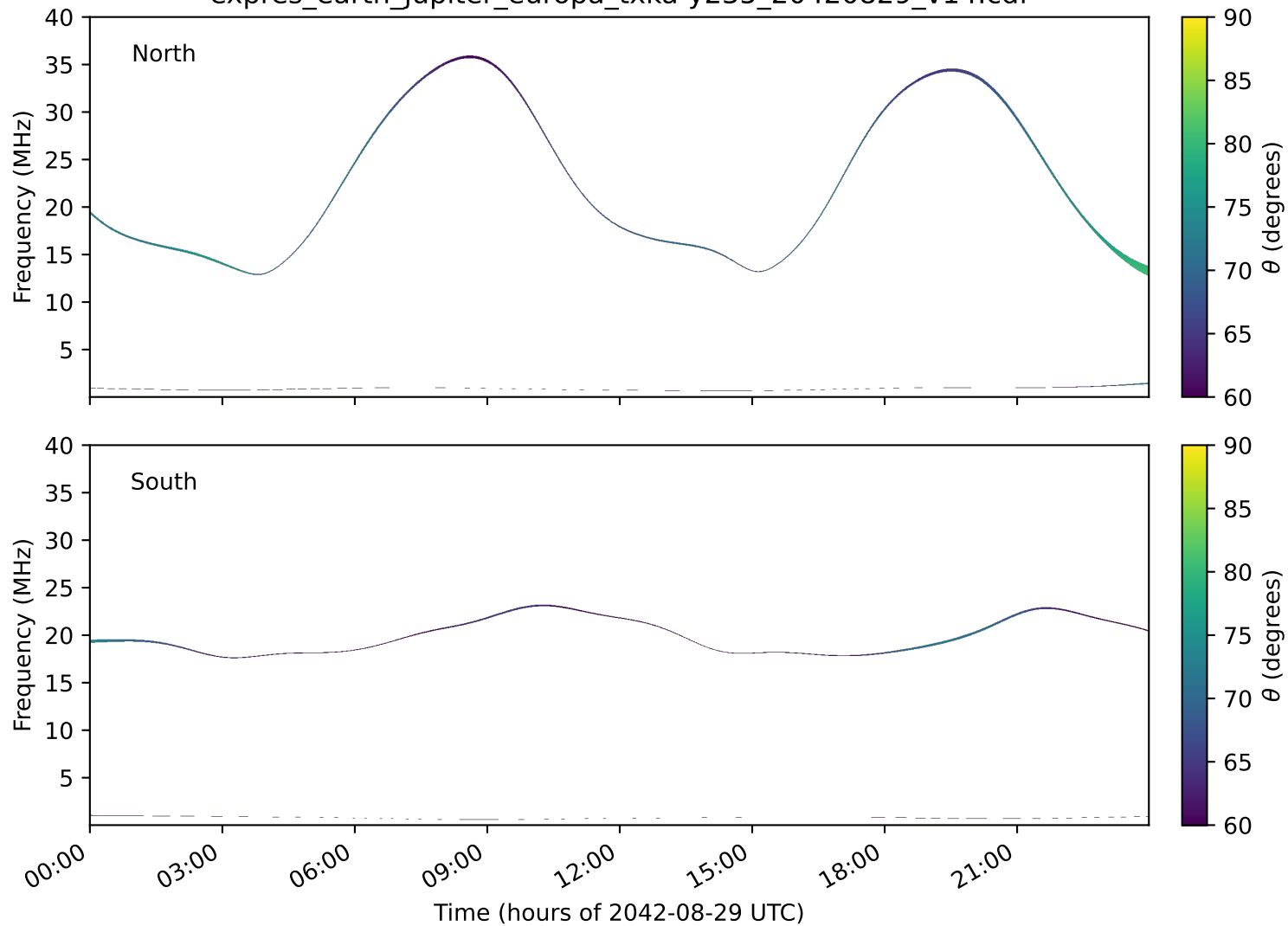
expres_earth_jupiter_europa_txka-y235_20420829_v14.cdf
