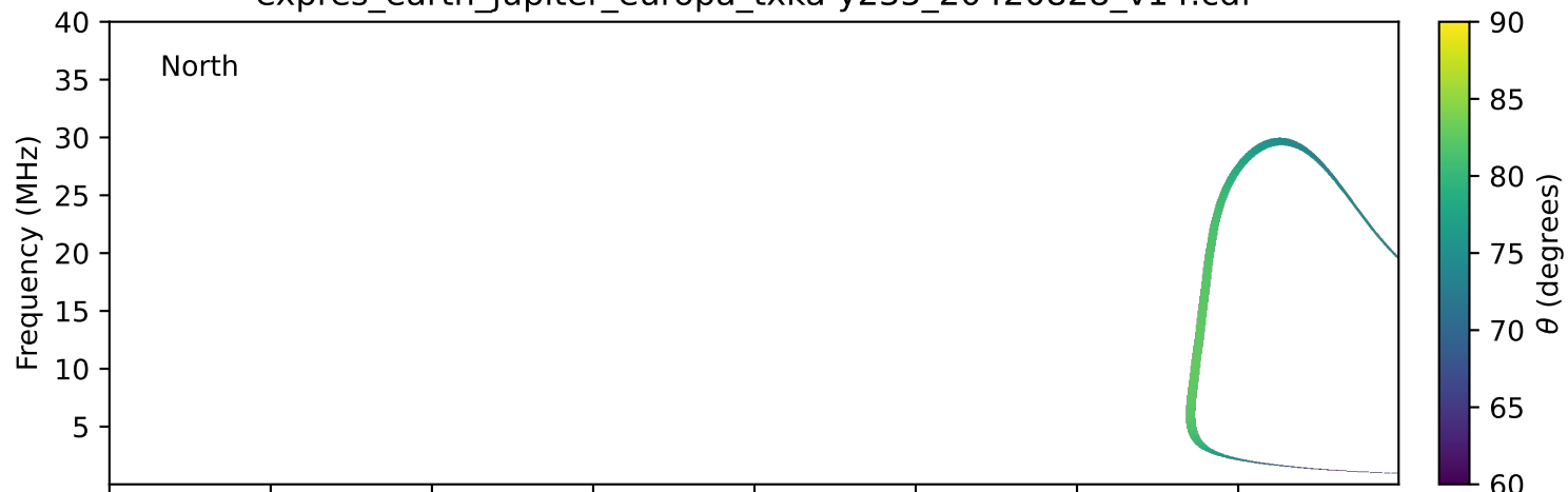
expres_earth_jupiter_europa_txka-y235_20420828_v14.cdf
