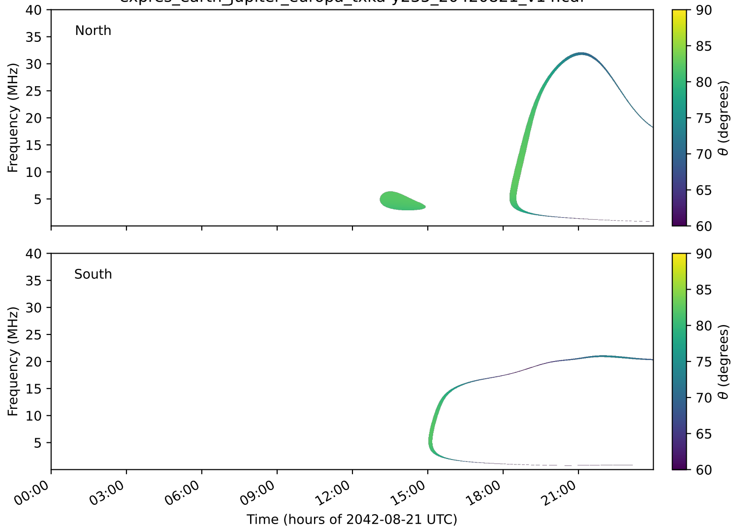
expres_earth_jupiter_europa_txka-y235_20420821_v14.cdf
