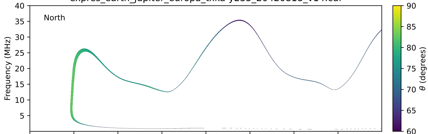
expres_earth_jupiter_europa_txka-y235_20420818_v14.cdf
