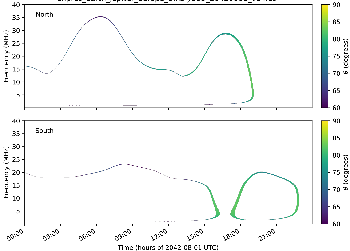
expres_earth_jupiter_europa_txka-y235_20420801_v14.cdf
