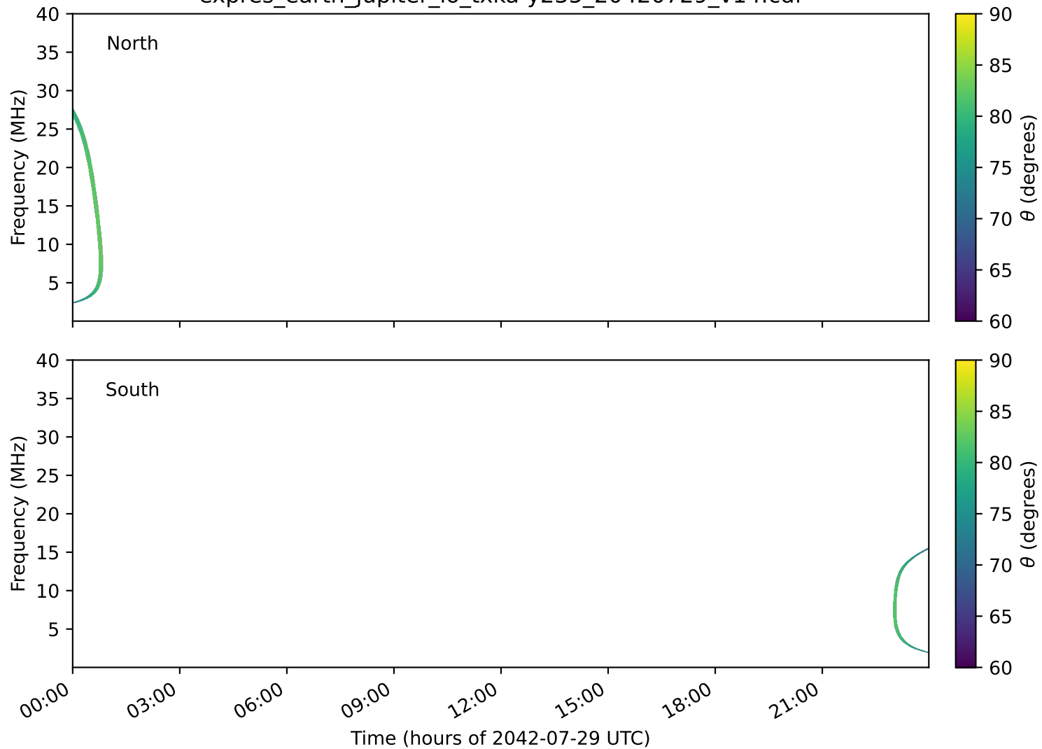
expres_earth_jupiter_io_txka-y235_20420729_v14.cdf
