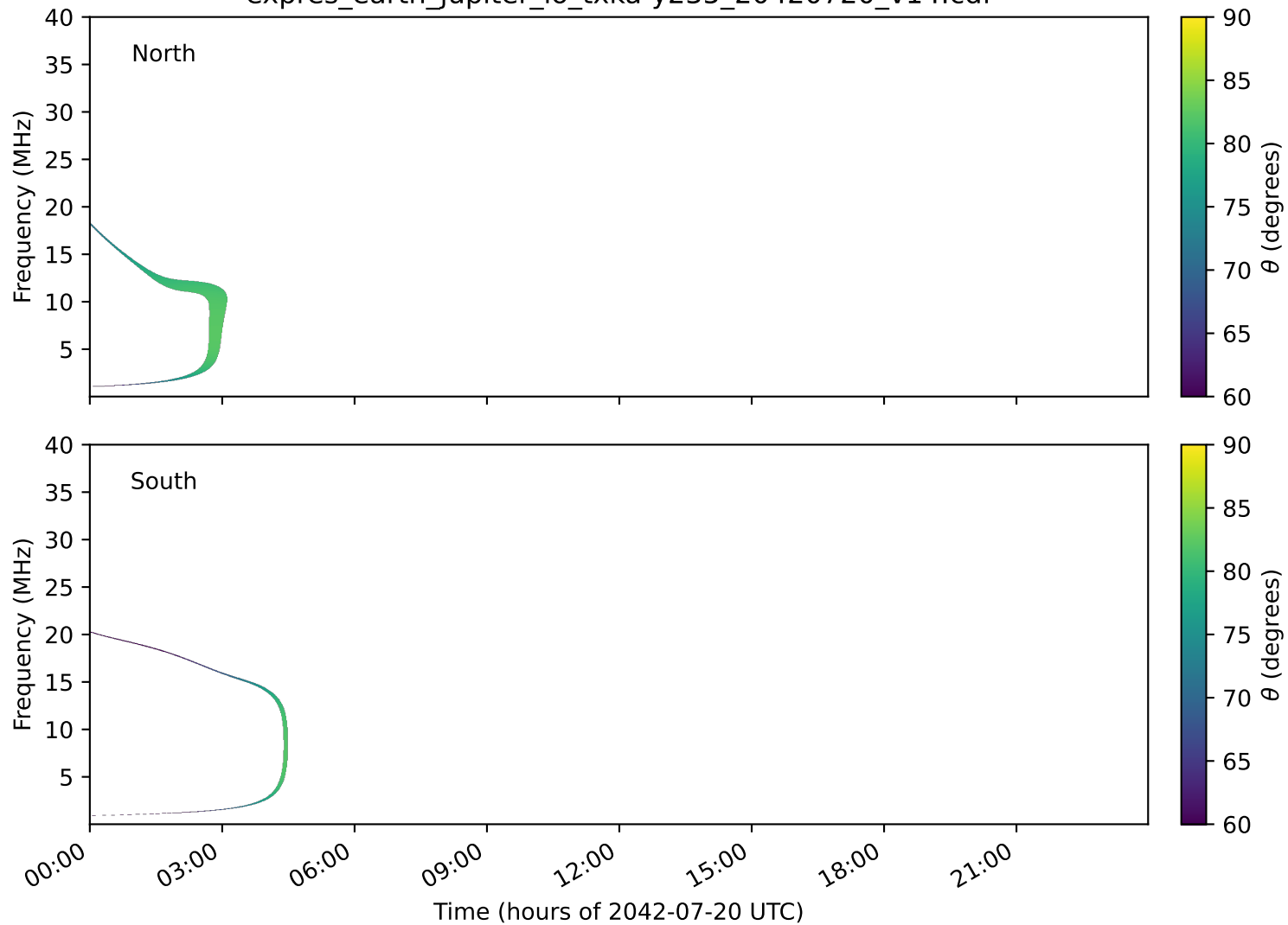
expres_earth_jupiter_io_txka-y235_20420720_v14.cdf
