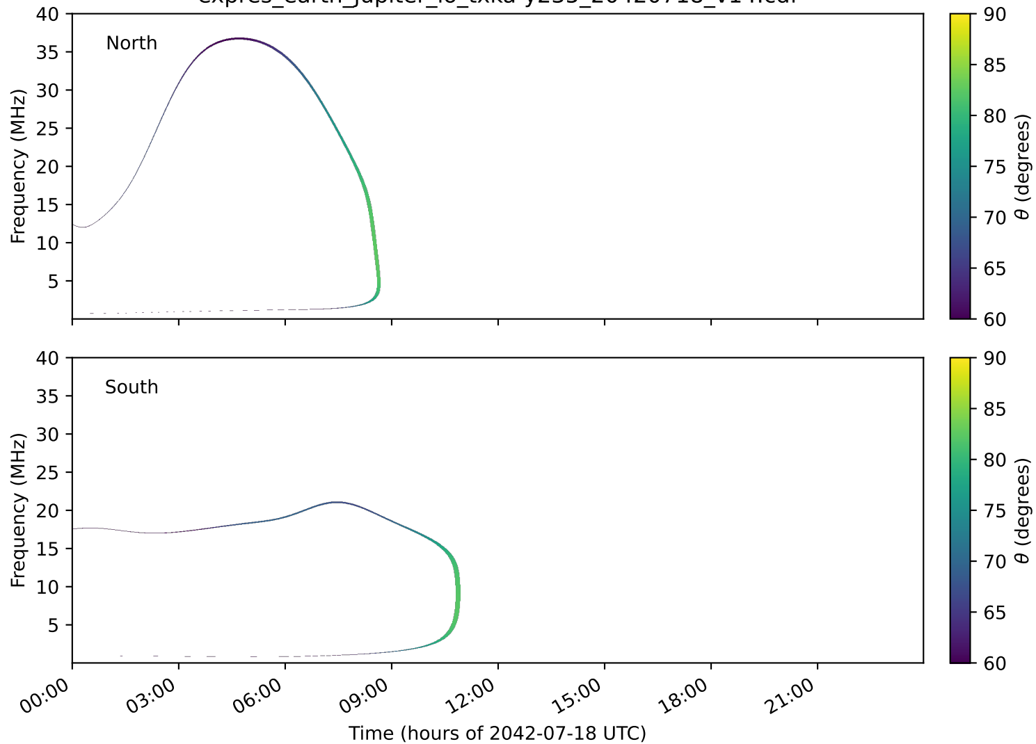
expres_earth_jupiter_io_txka-y235_20420718_v14.cdf
