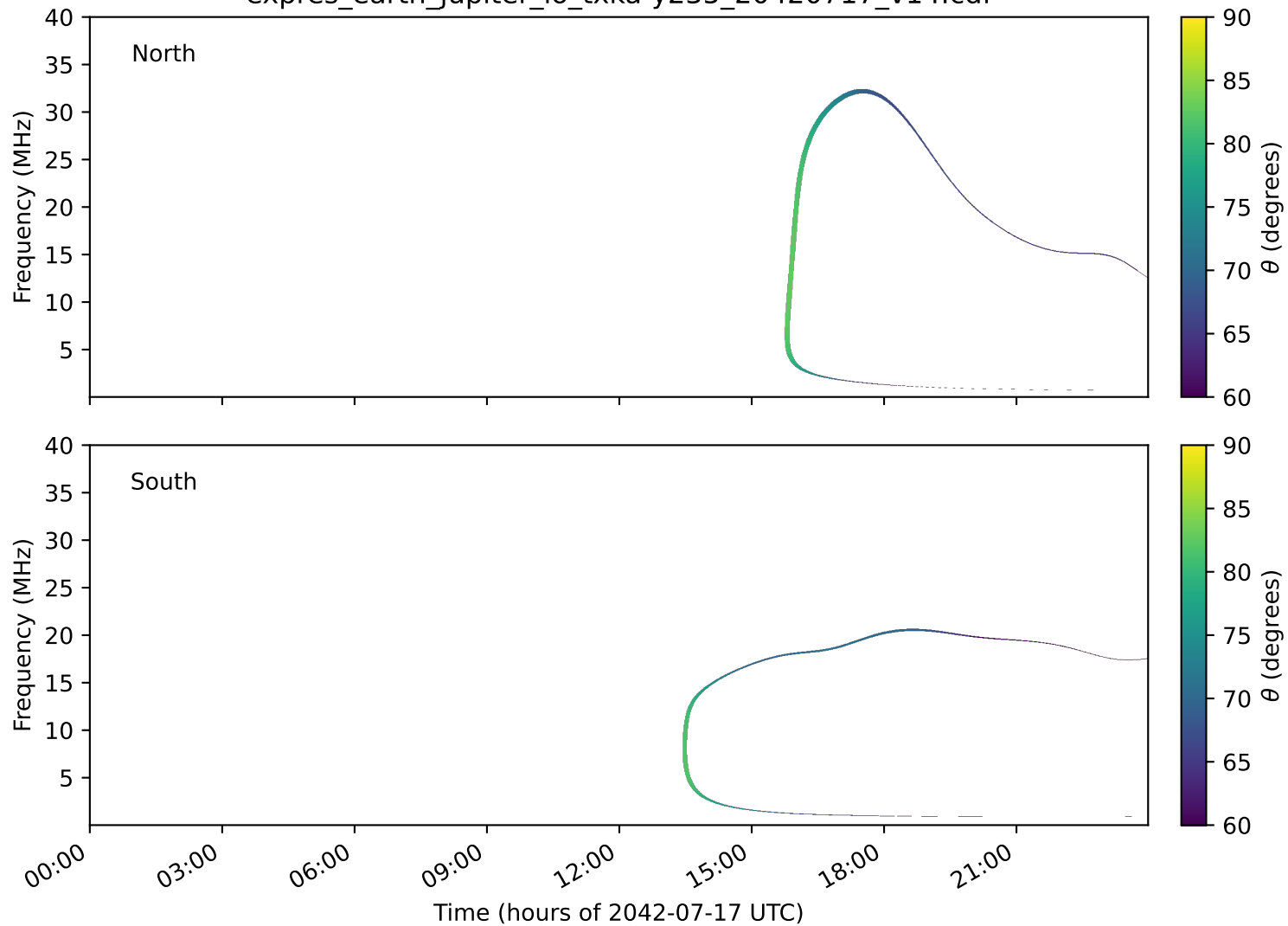
expres_earth_jupiter_io_txka-y235_20420717_v14.cdf
