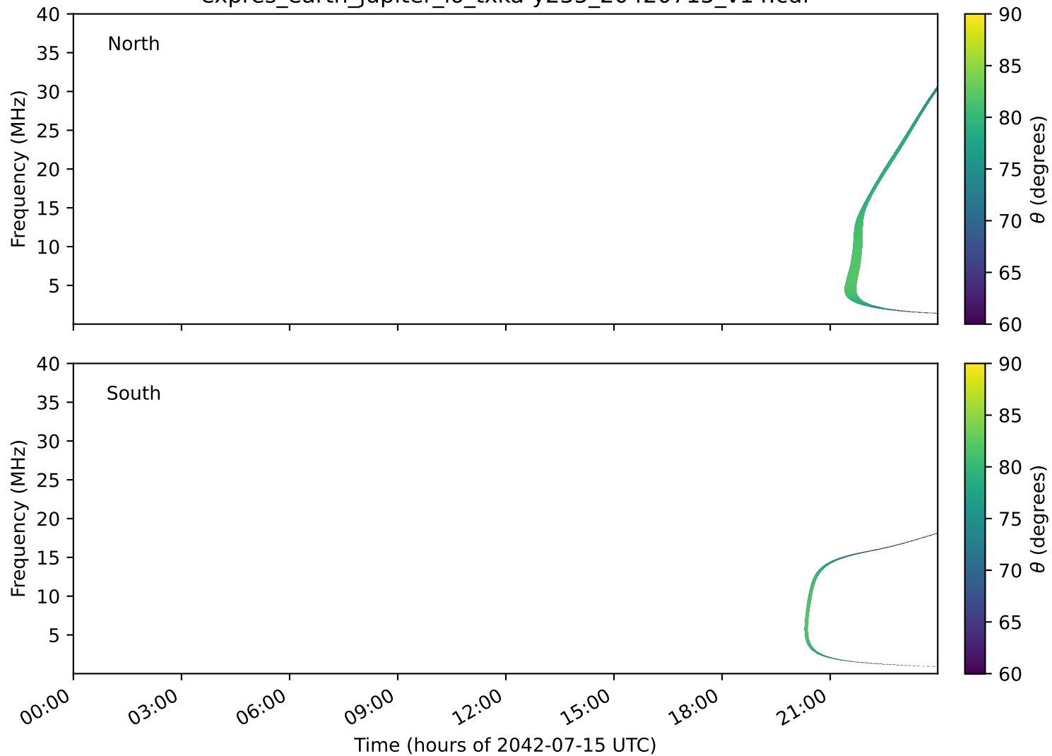
expres_earth_jupiter_io_txka-y235_20420715_v14.cdf
