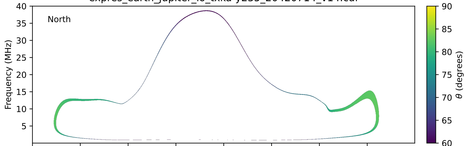
expres_earth_jupiter_io_txka-y235_20420714_v14.cdf
