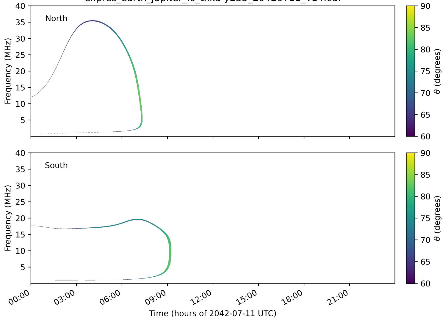
expres_earth_jupiter_io_txka-y235_20420711_v14.cdf
