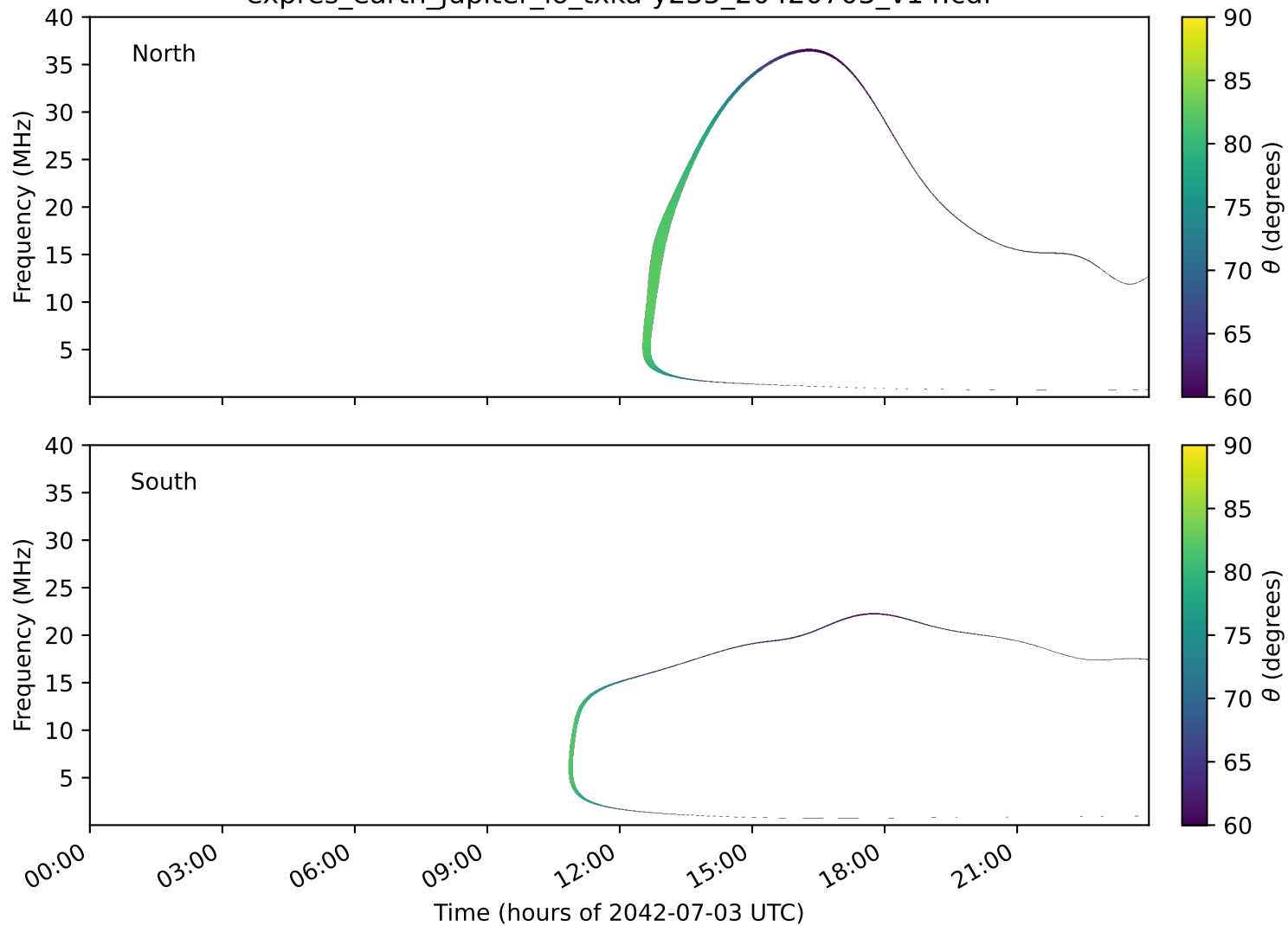
expres_earth_jupiter_io_txka-y235_20420703_v14.cdf
