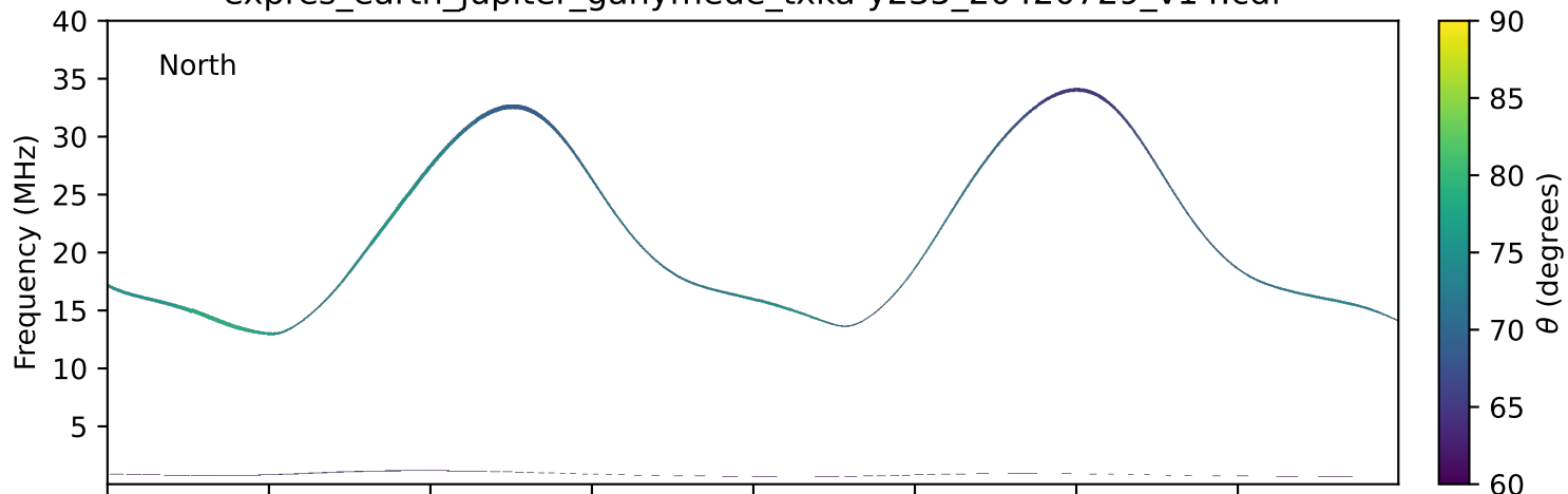
expres_earth_jupiter_ganymede_txka-y235_20420729_v14.cdf
