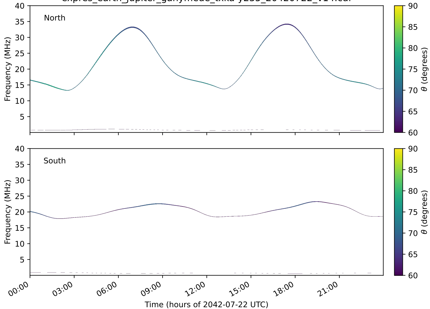
expres_earth_jupiter_ganymede_txka-y235_20420722_v14.cdf
