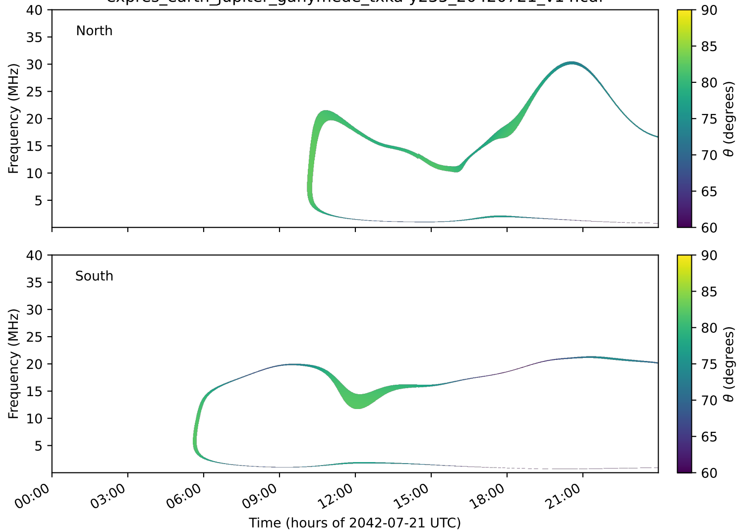
expres_earth_jupiter_ganymede_txka-y235_20420721_v14.cdf
