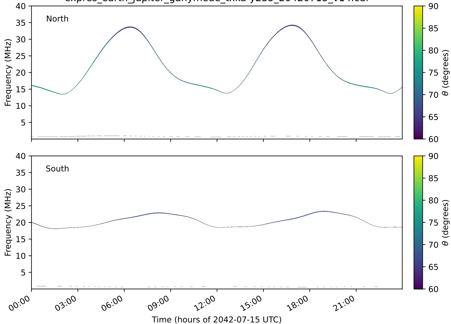
expres_earth_jupiter_ganymede_txka-y235_20420715_v14.cdf
