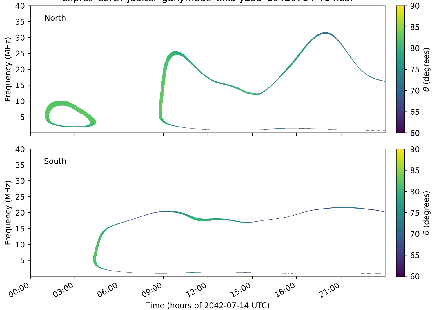
expres_earth_jupiter_ganymede_txka-y235_20420714_v14.cdf
