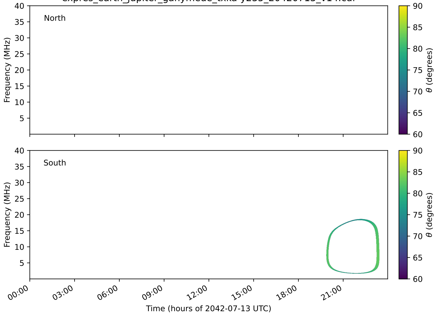
expres_earth_jupiter_ganymede_txka-y235_20420713_v14.cdf
