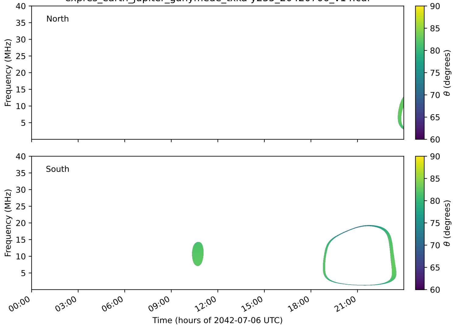
expres_earth_jupiter_ganymede_txka-y235_20420706_v14.cdf
