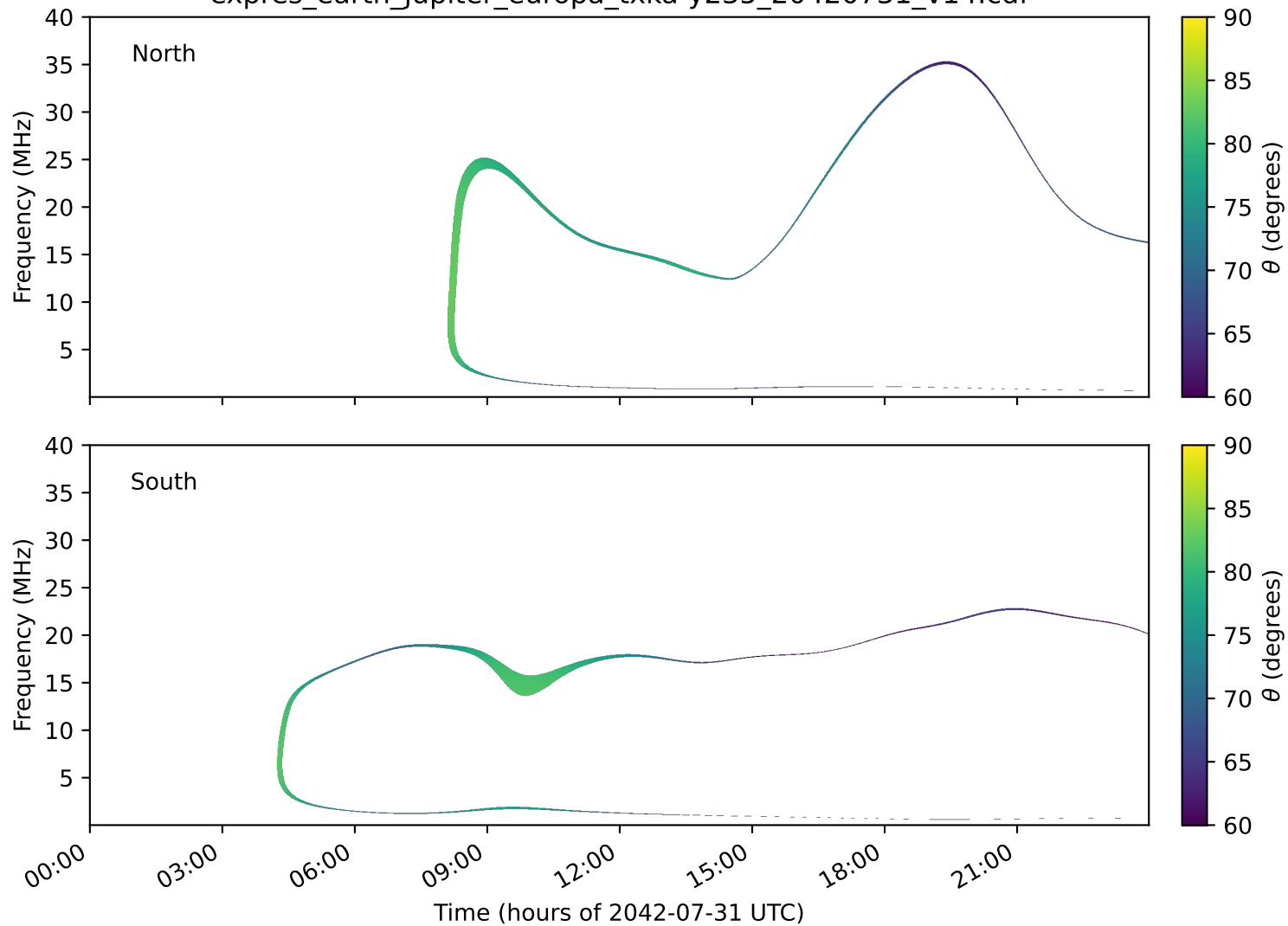
expres_earth_jupiter_europa_txka-y235_20420731_v14.cdf
