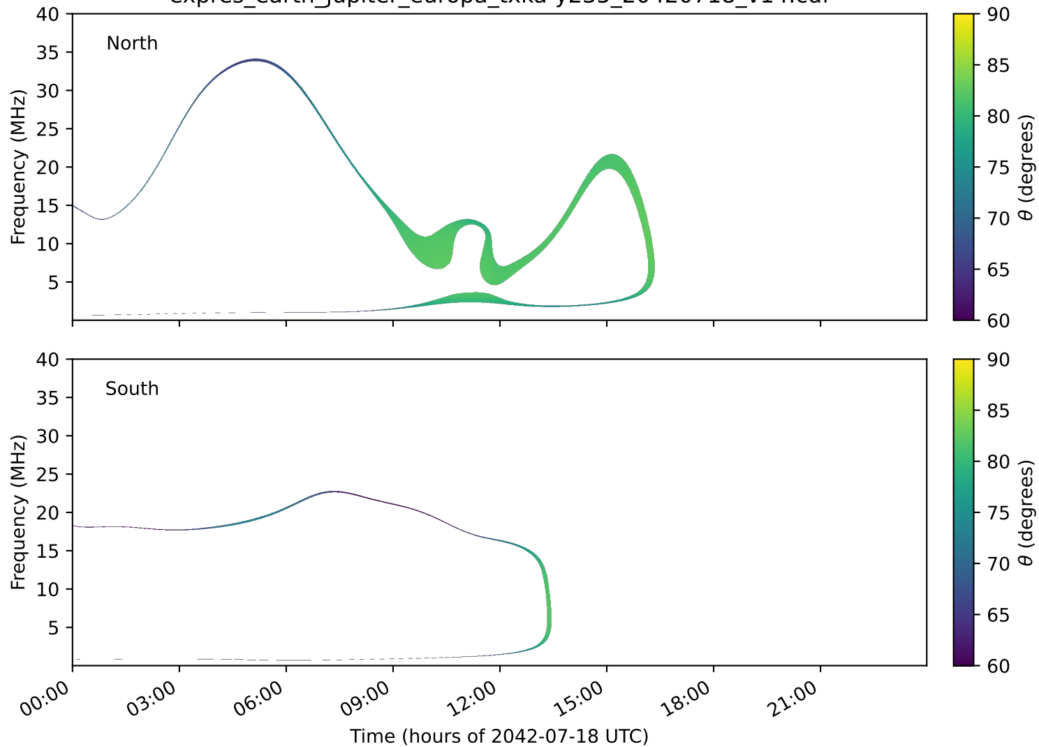
expres_earth_jupiter_europa_txka-y235_20420718_v14.cdf
