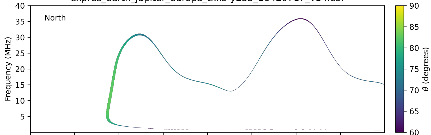
expres_earth_jupiter_europa_txka-y235_20420717_v14.cdf
