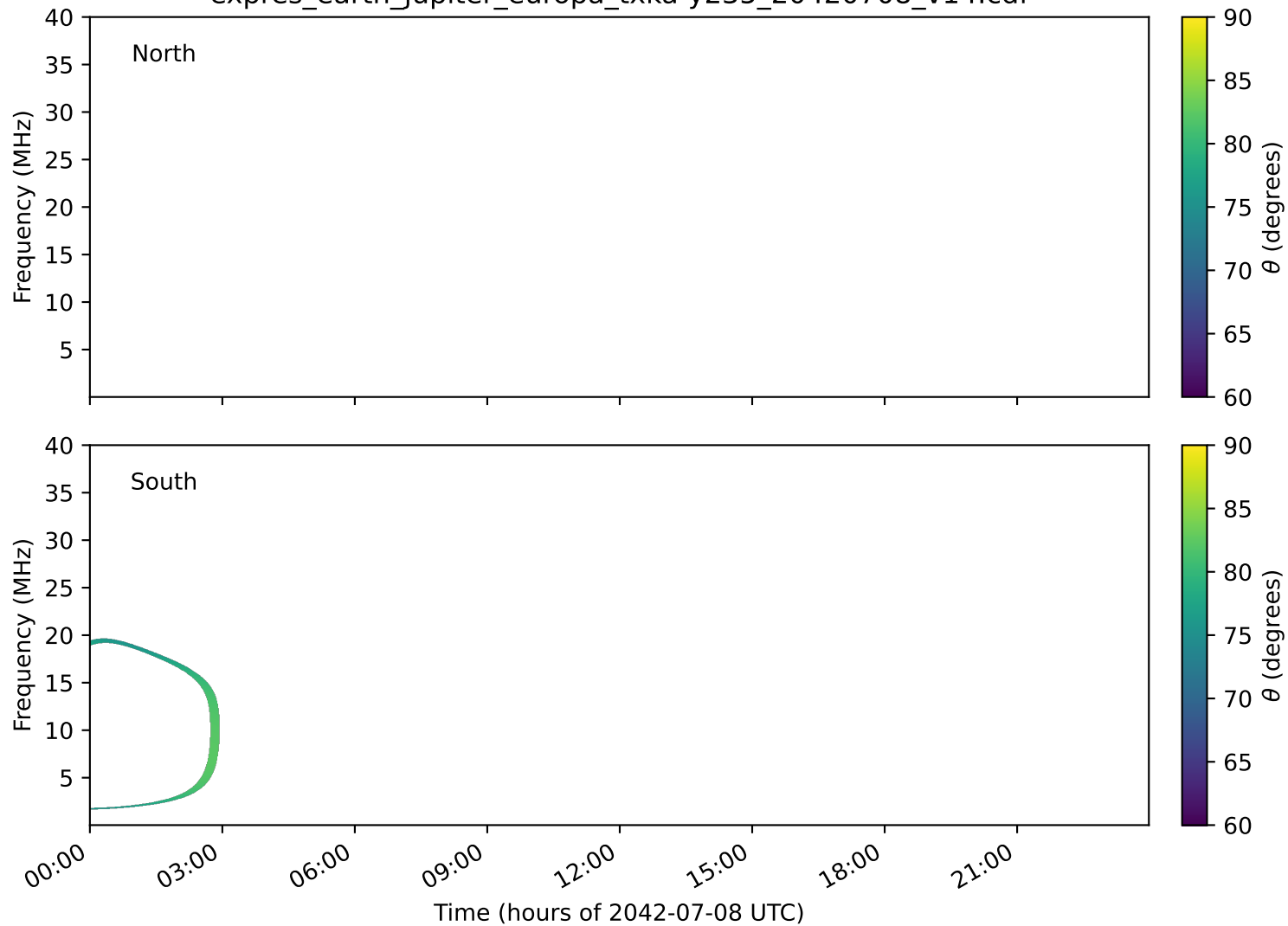
expres_earth_jupiter_europa_txka-y235_20420708_v14.cdf
