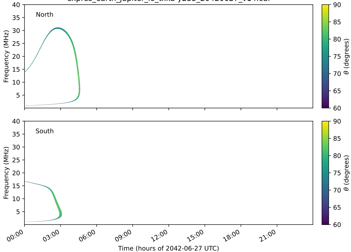
expres_earth_jupiter_io_txka-y235_20420627_v14.cdf
