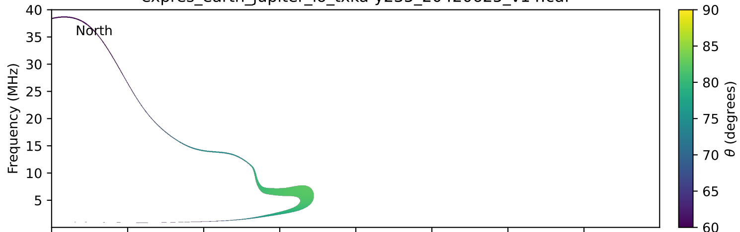
expres_earth_jupiter_io_txka-y235_20420625_v14.cdf
