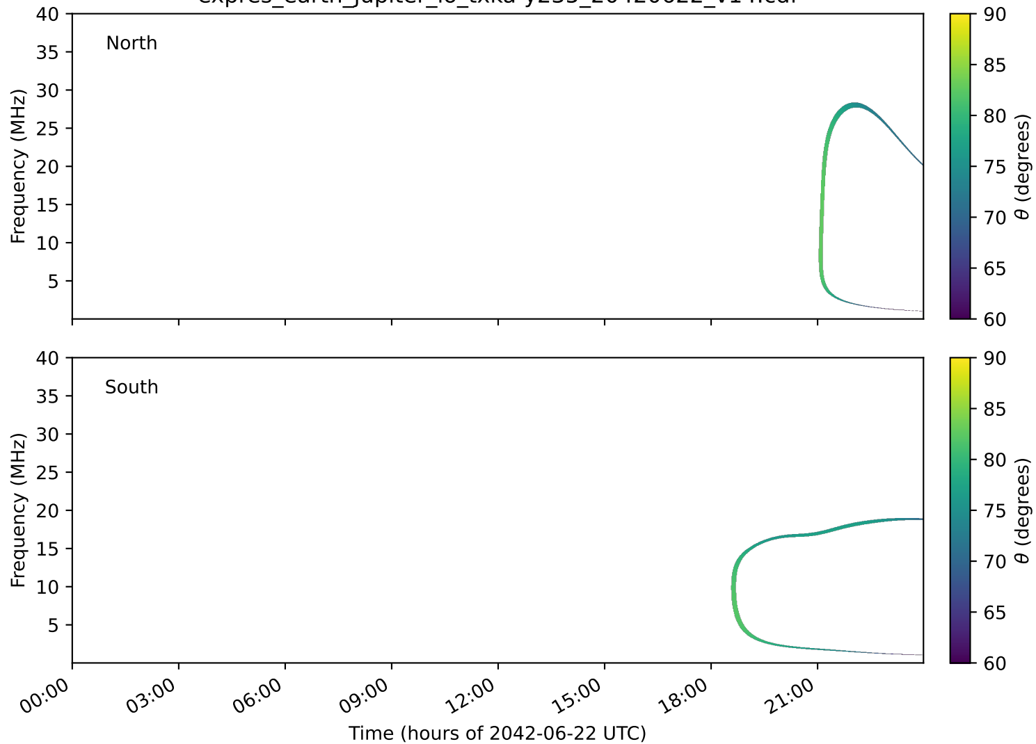
expres_earth_jupiter_io_txka-y235_20420622_v14.cdf
