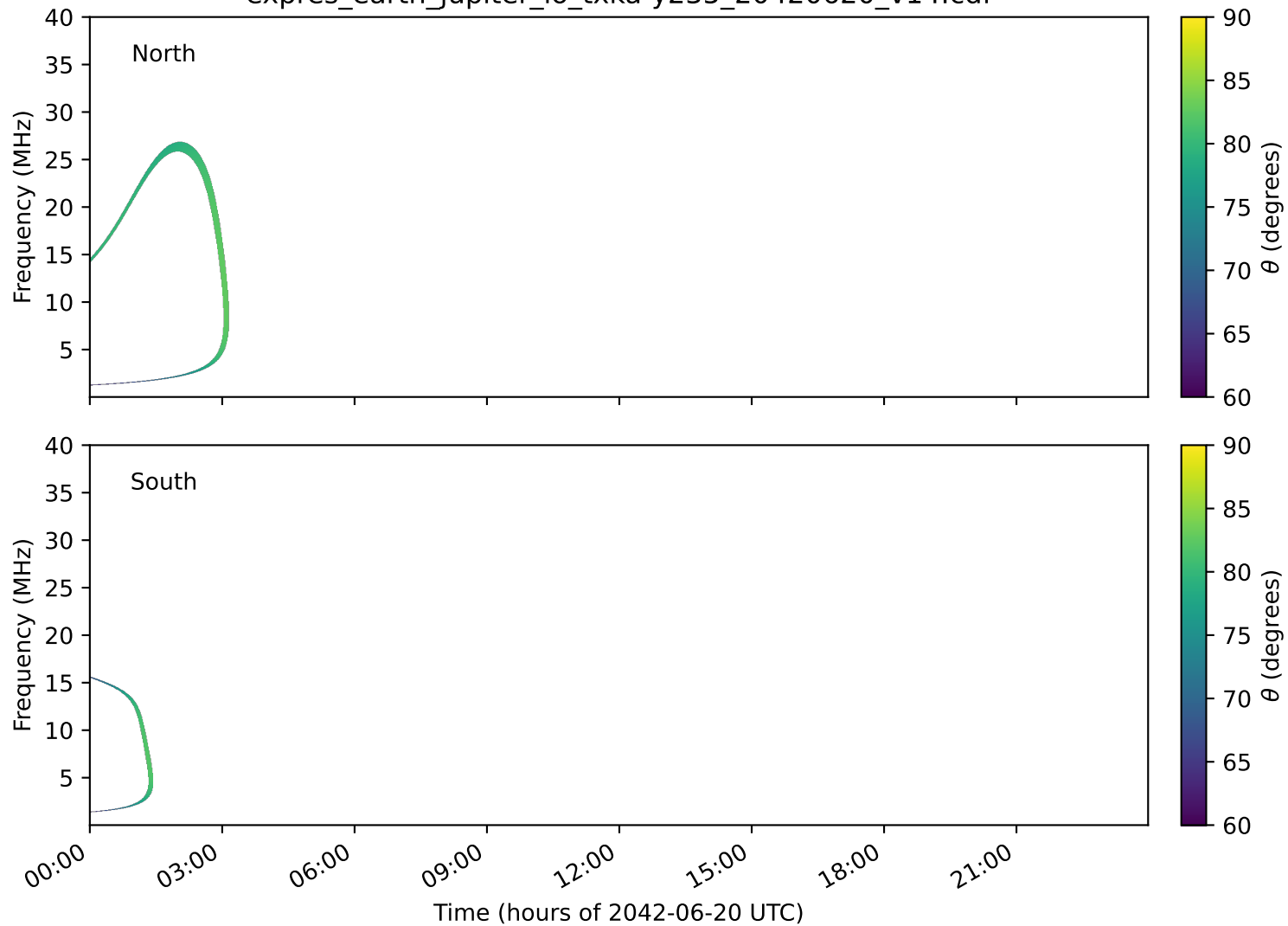
expres_earth_jupiter_io_txka-y235_20420620_v14.cdf
