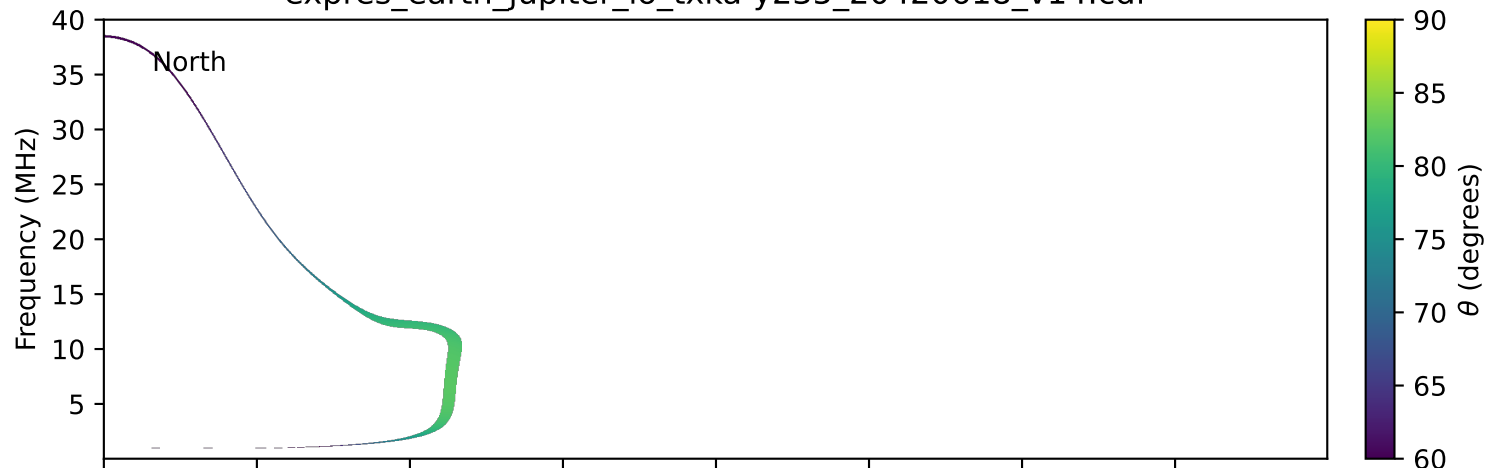
expres_earth_jupiter_io_txka-y235_20420618_v14.cdf
