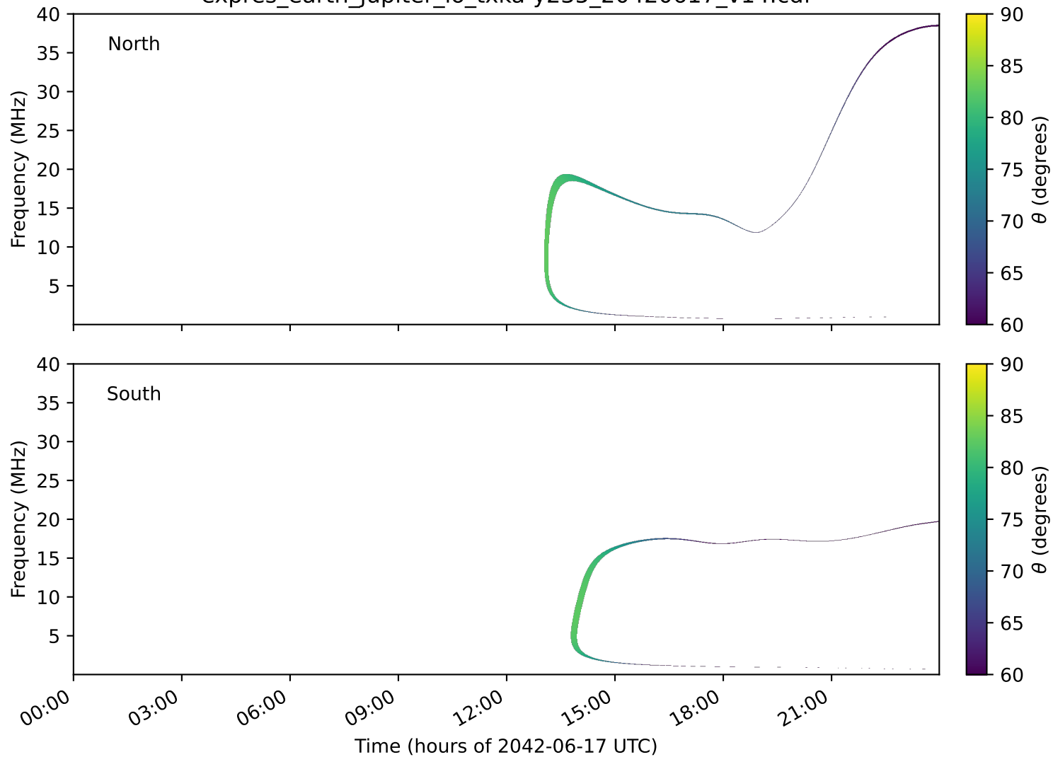
expres_earth_jupiter_io_txka-y235_20420617_v14.cdf
