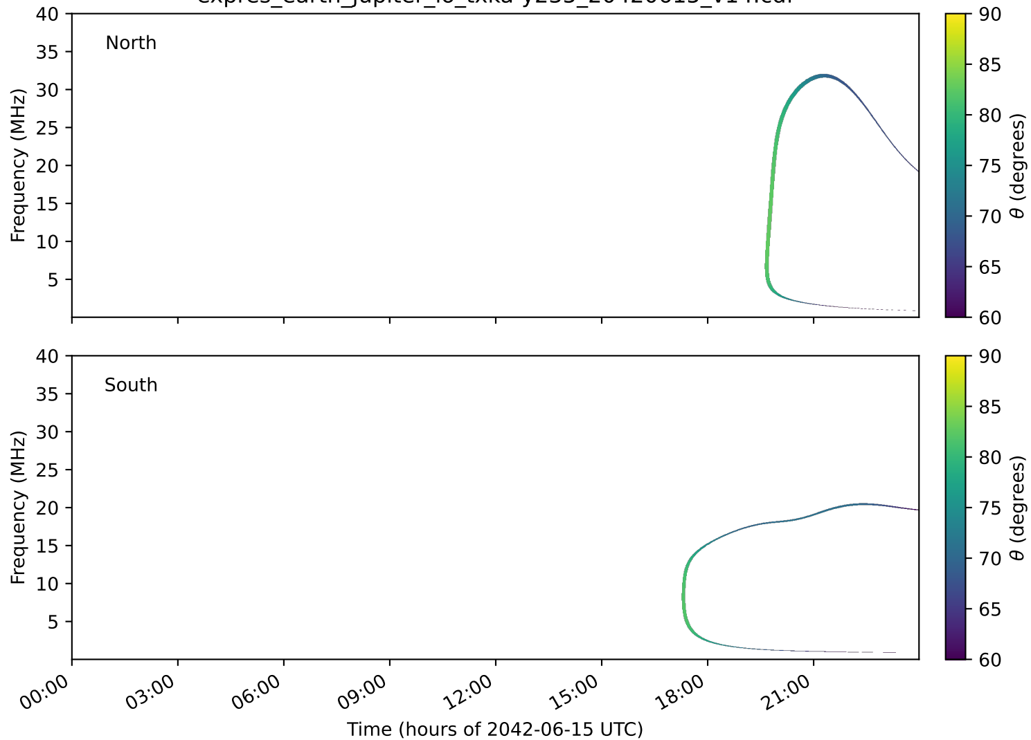
expres_earth_jupiter_io_txka-y235_20420615_v14.cdf
