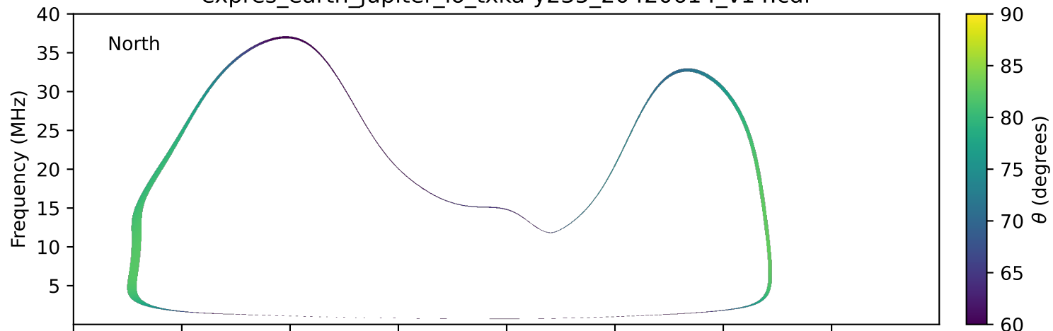
expres_earth_jupiter_io_txka-y235_20420614_v14.cdf
