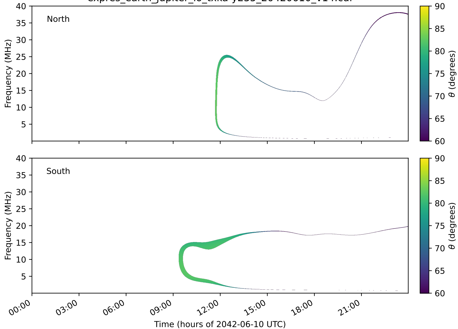
expres_earth_jupiter_io_txka-y235_20420610_v14.cdf
