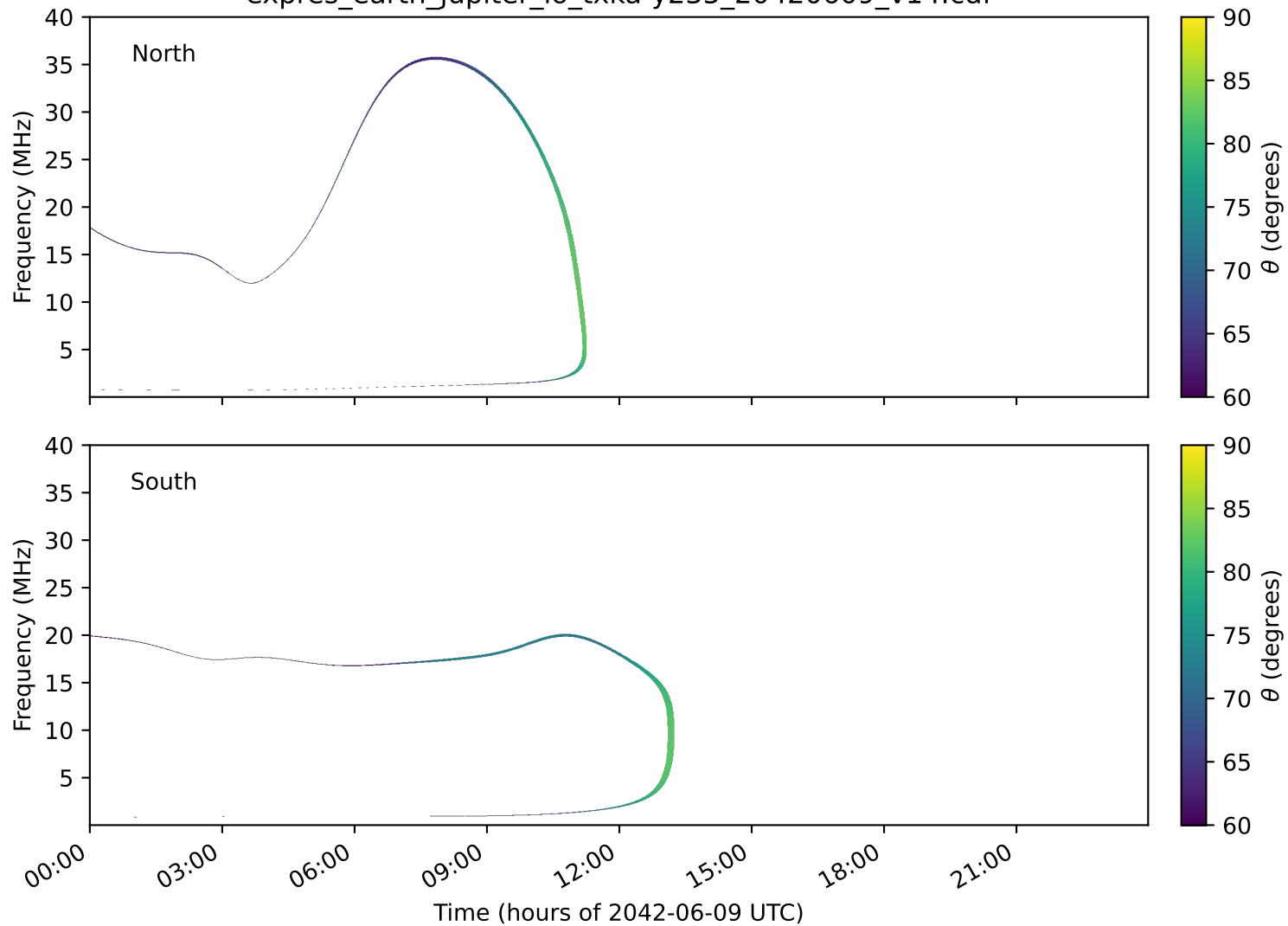
expres_earth_jupiter_io_txka-y235_20420609_v14.cdf
