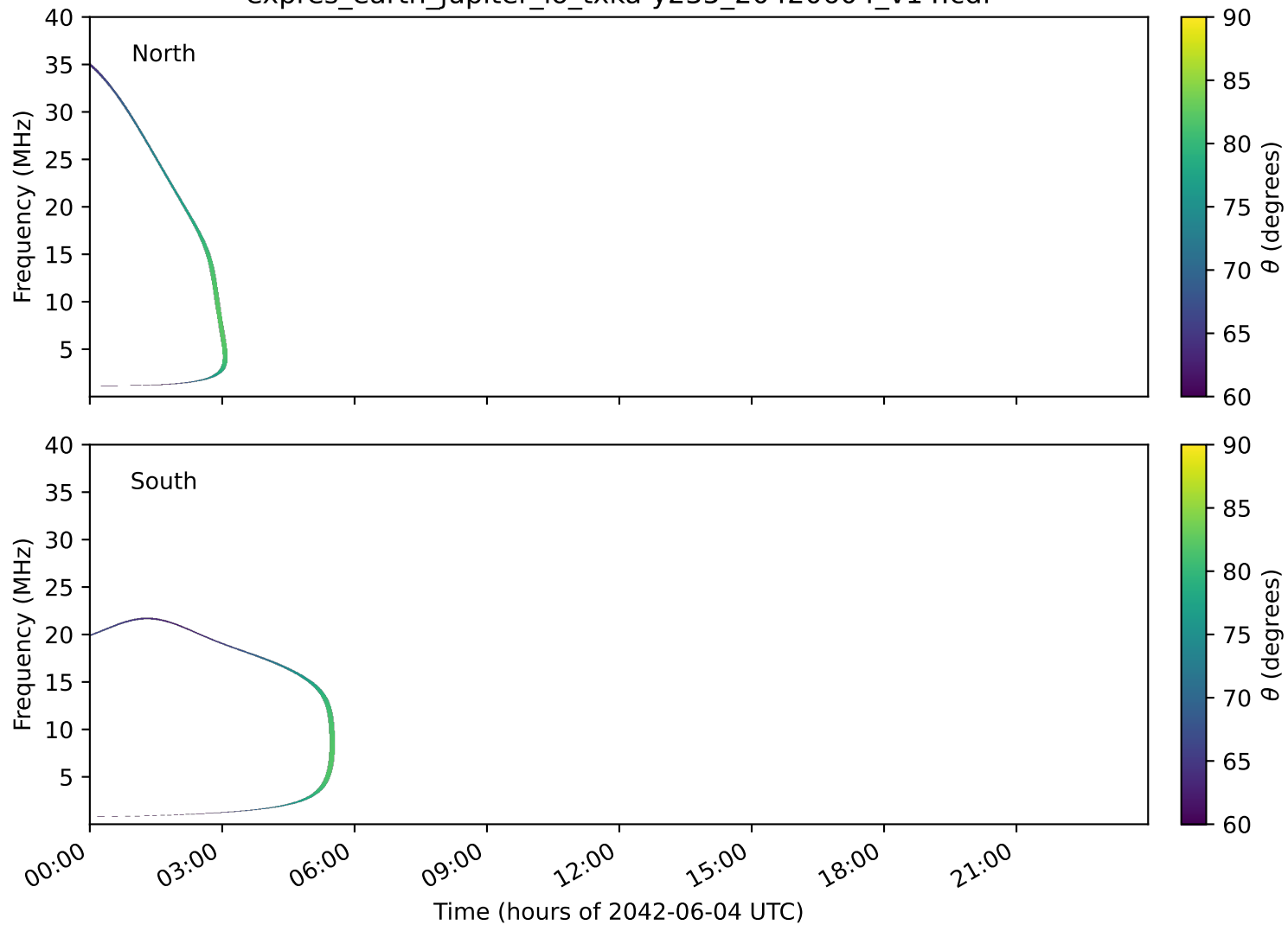
expres_earth_jupiter_io_txka-y235_20420604_v14.cdf
