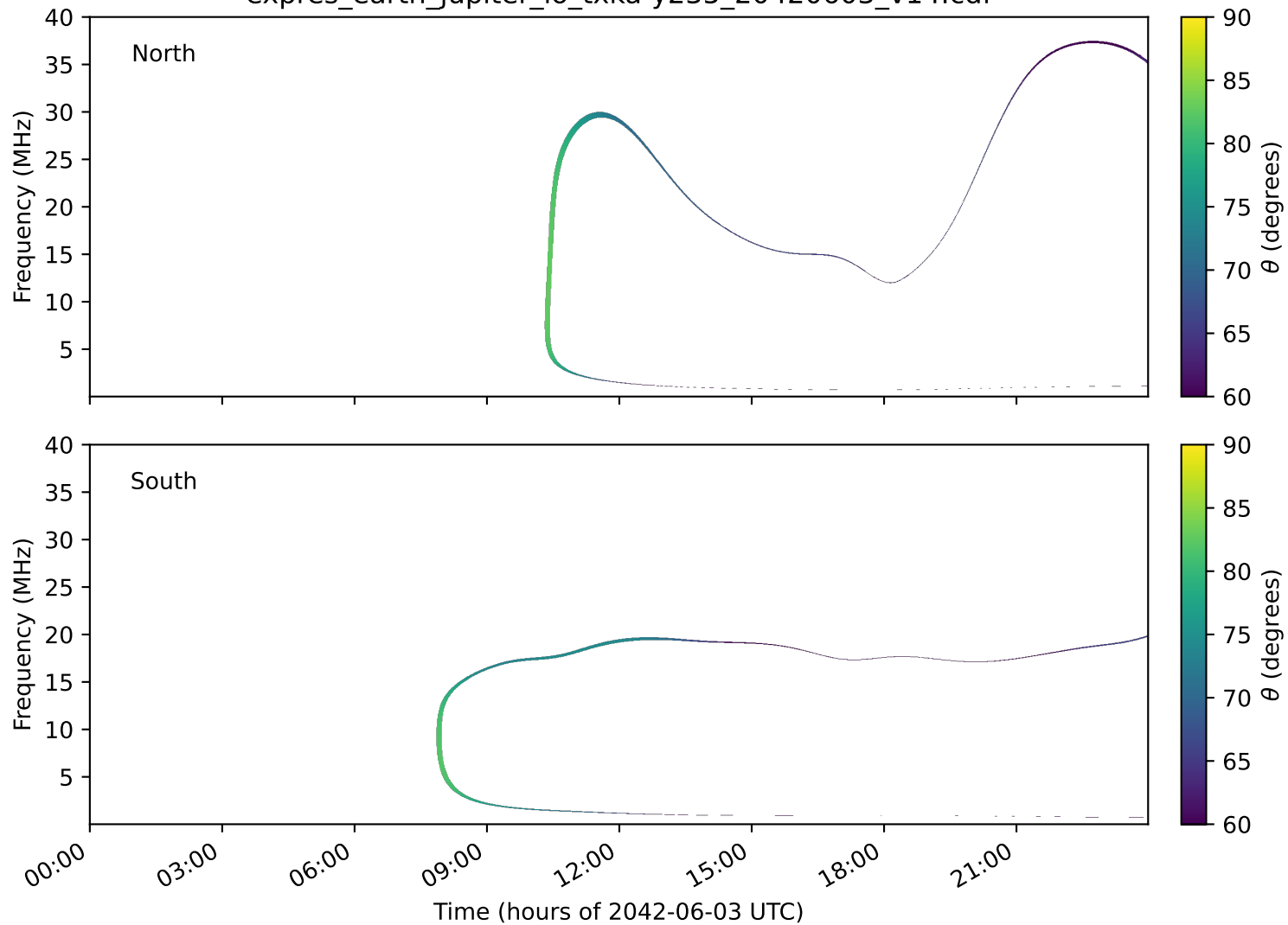
expres_earth_jupiter_io_txka-y235_20420603_v14.cdf
