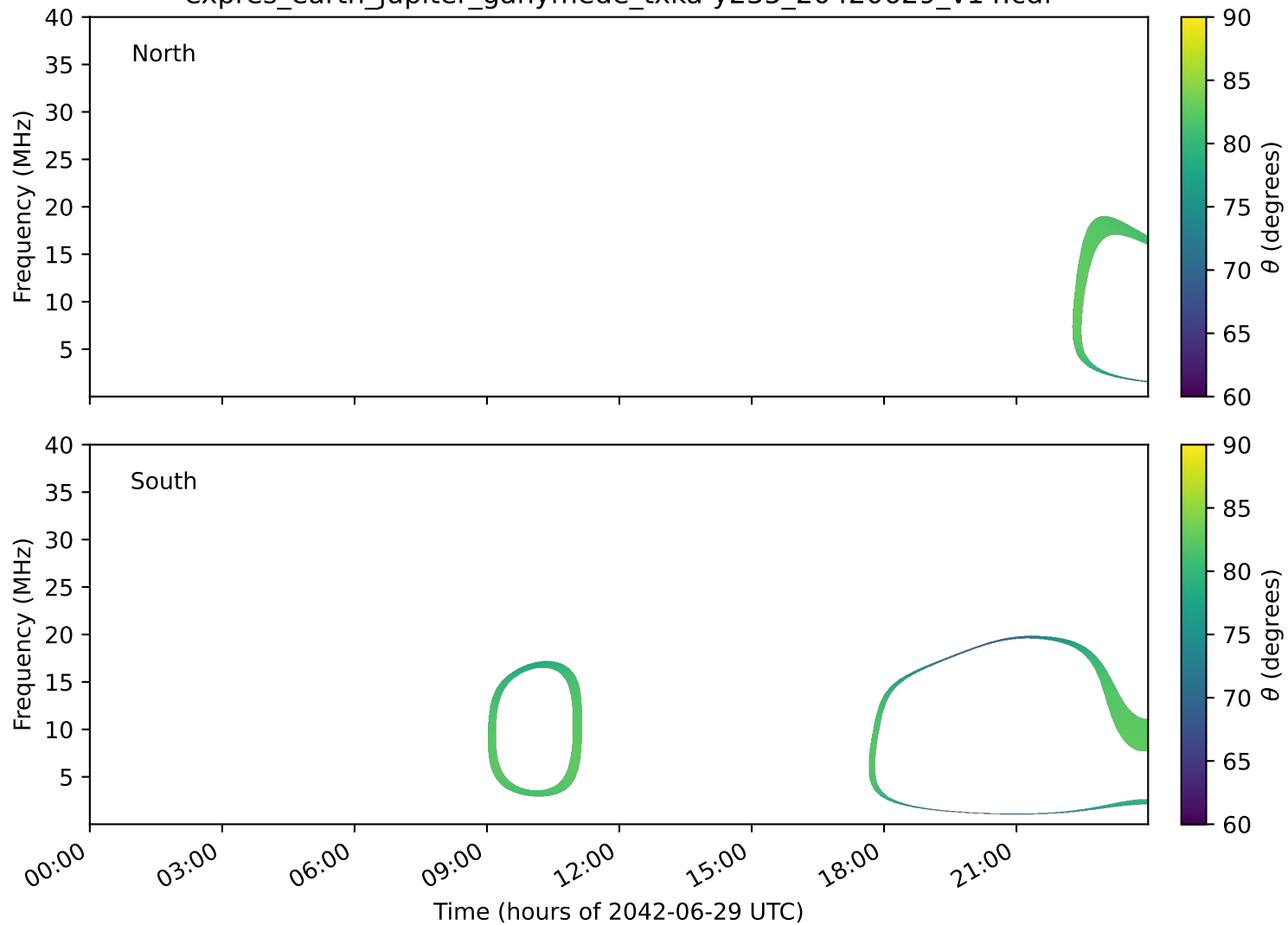
expres_earth_jupiter_ganymede_txka-y235_20420629_v14.cdf
