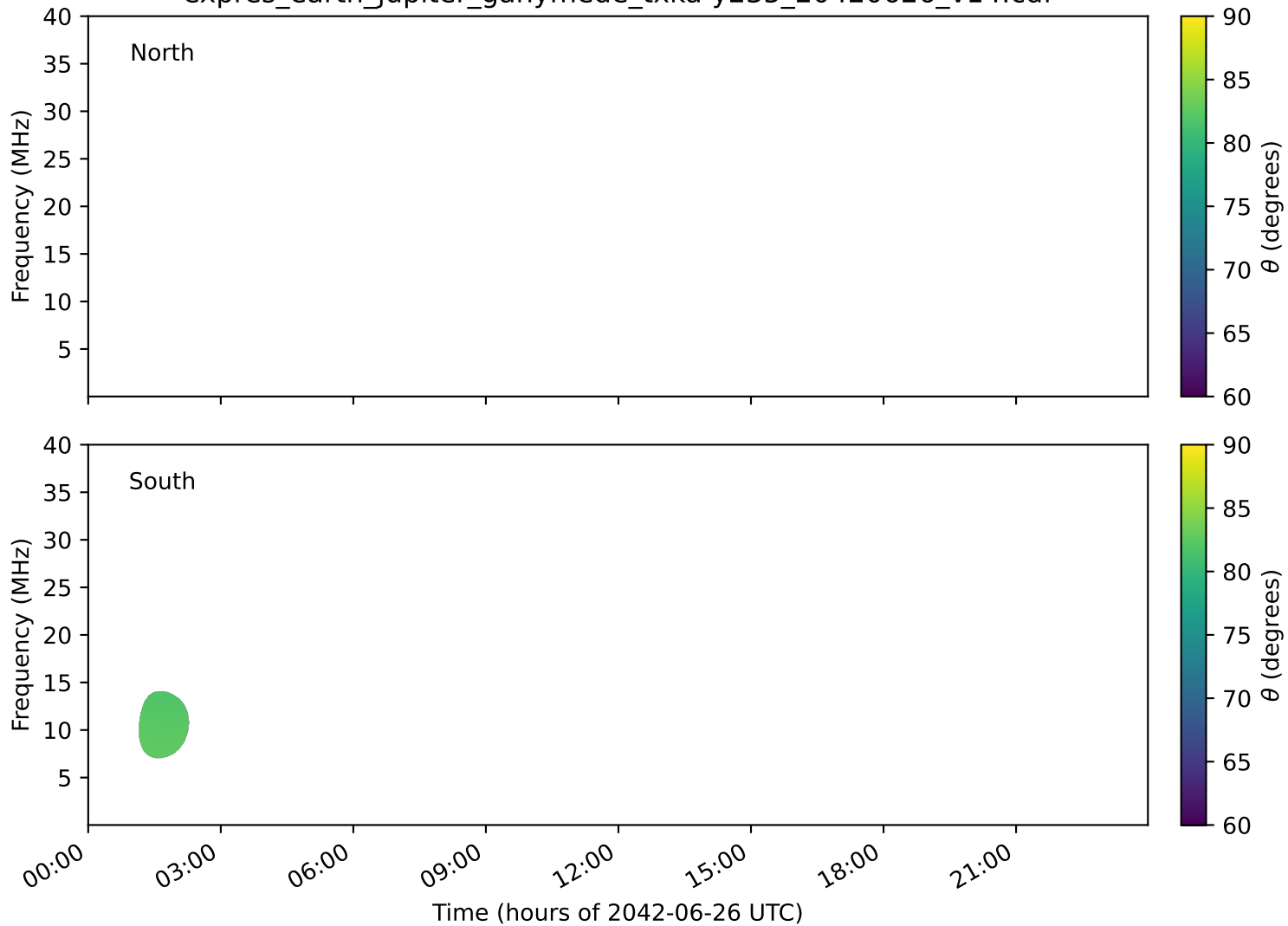
expres_earth_jupiter_ganymede_txka-y235_20420626_v14.cdf
