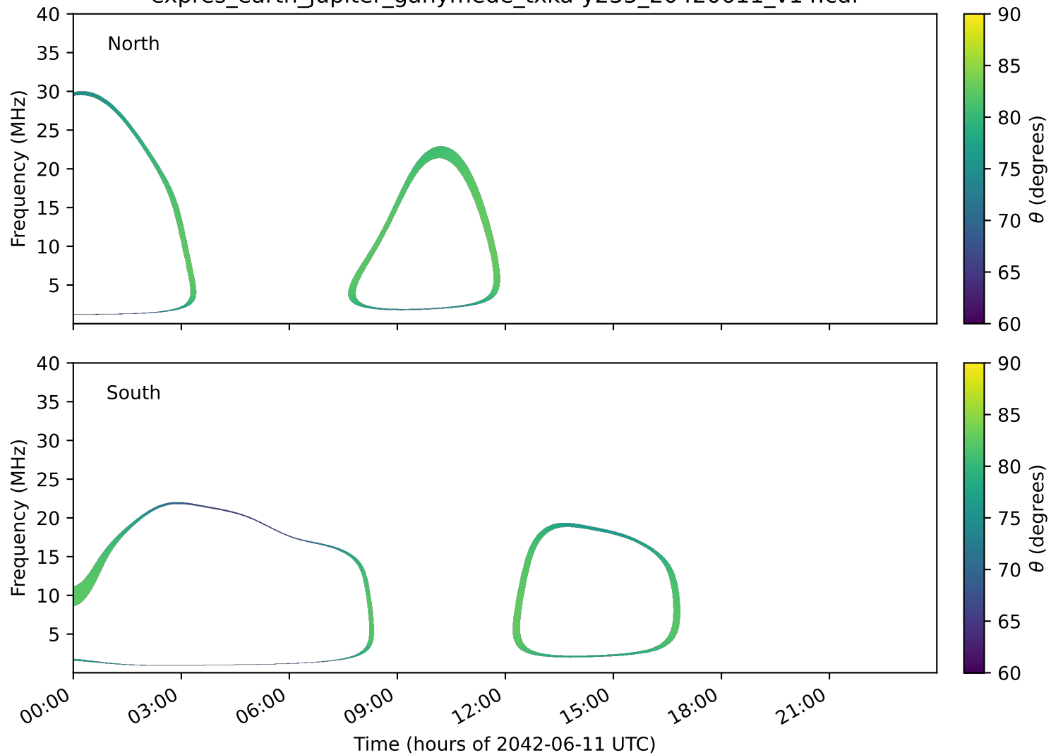
expres_earth_jupiter_ganymede_txka-y235_20420611_v14.cdf
