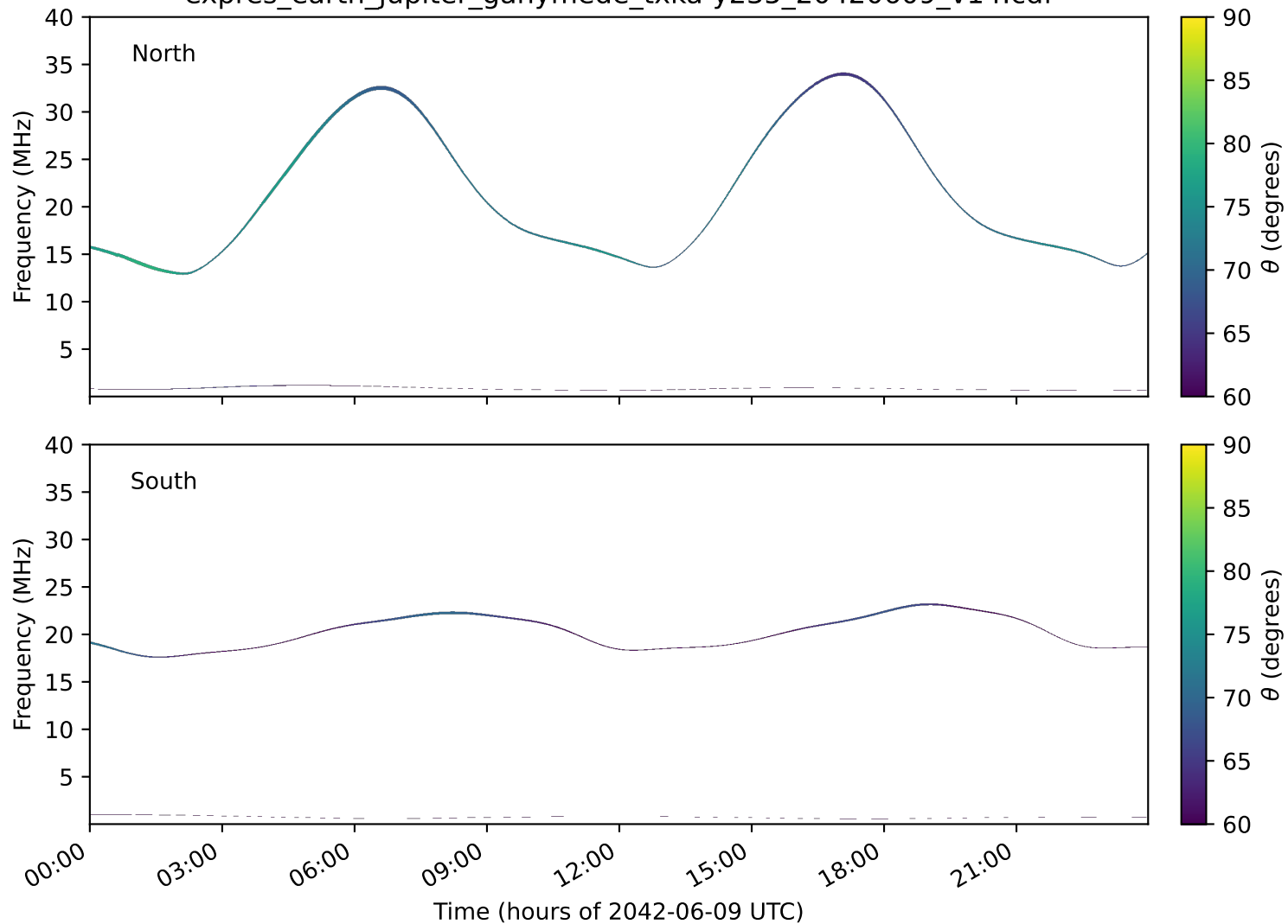
expres_earth_jupiter_ganymede_txka-y235_20420609_v14.cdf
