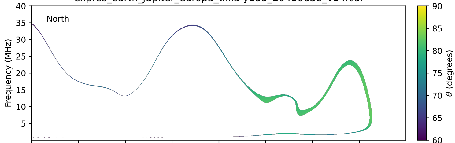
expres_earth_jupiter_europa_txka-y235_20420630_v14.cdf
